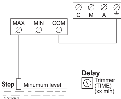
Connection diagram with timed level probe
