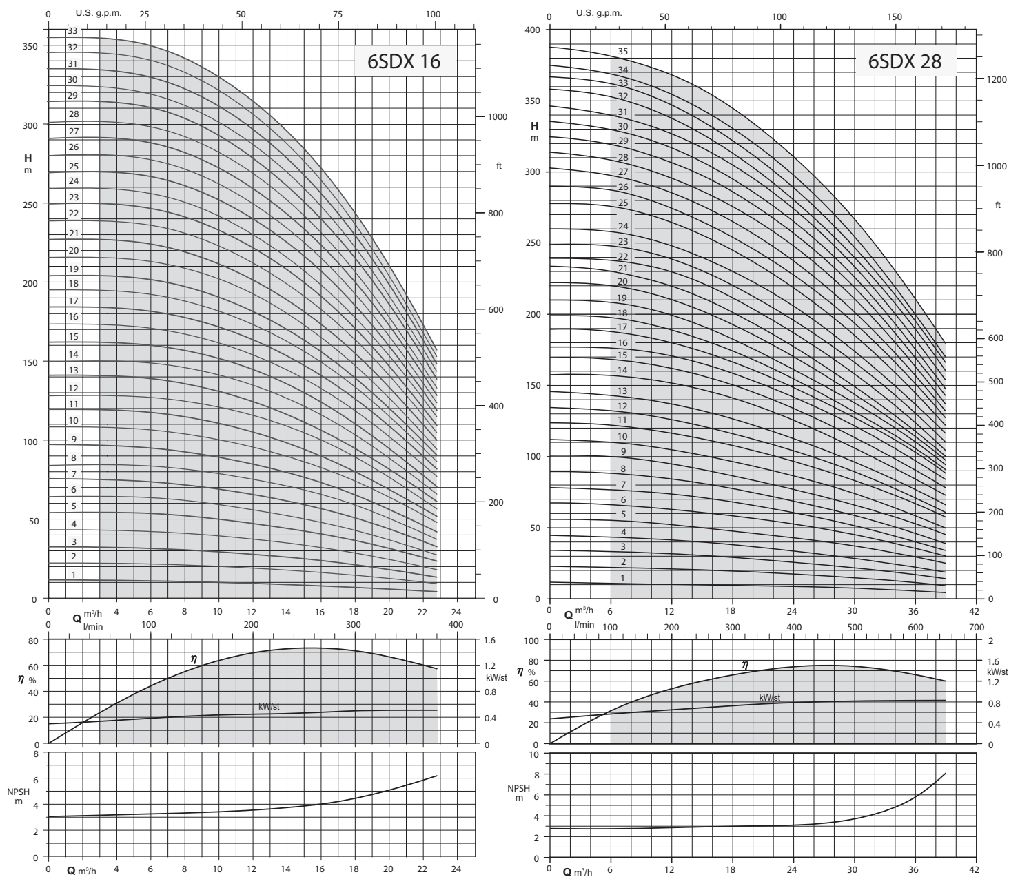
Coverage chart n \approx 2900 rpm
