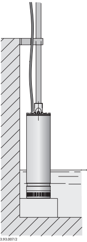
Fig. 3 Pompa sospesa Pump in the suspended position Pompe suspendue
