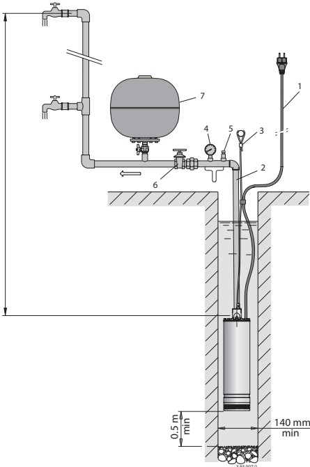
Fig. 3 Pompa sospesa Pump in the suspended position Pompe suspendue
