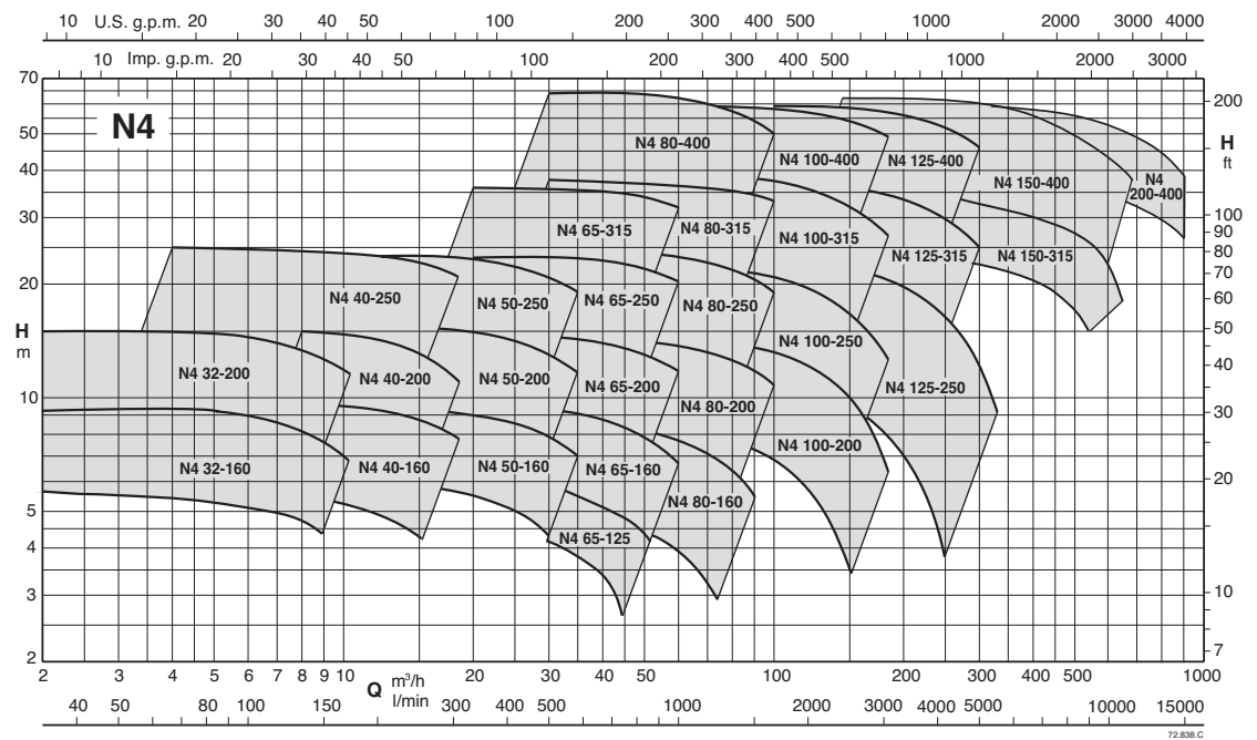
Performance n ≈ 1750 1/min
