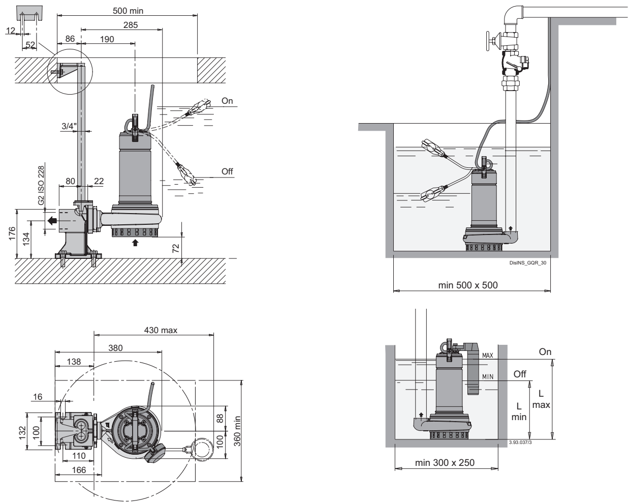
Installation examples with vertical magnetic float switch
