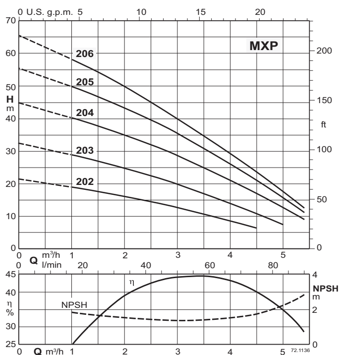
Characteristic curves n \approx 2800 1/min
