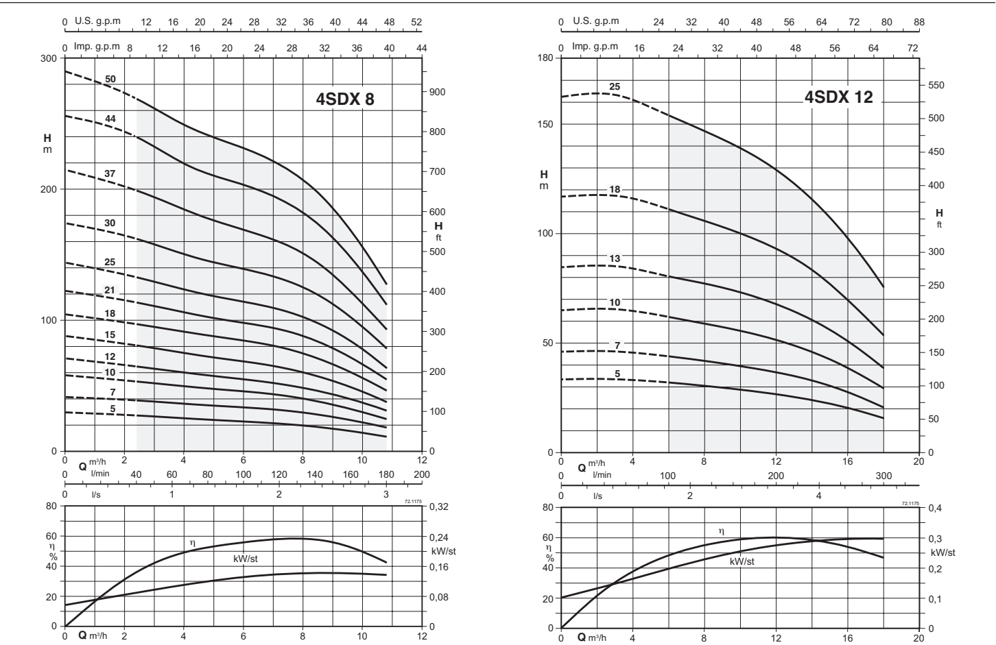
Coverage chart n ≈ 2900 rpm
