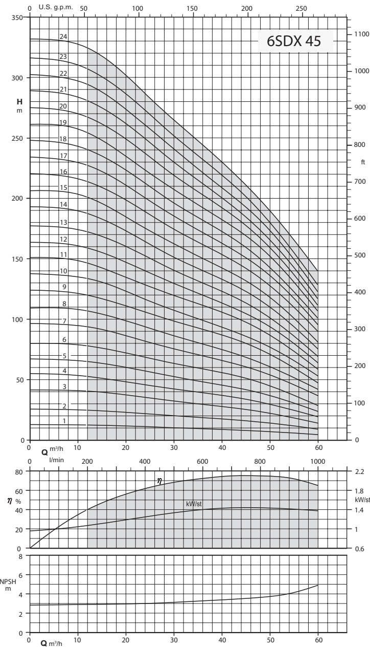
Coverage chart n \approx 2900 rpm
