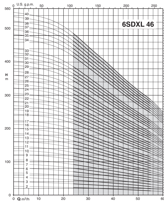
Coverage chart n \approx 2900 rpm
