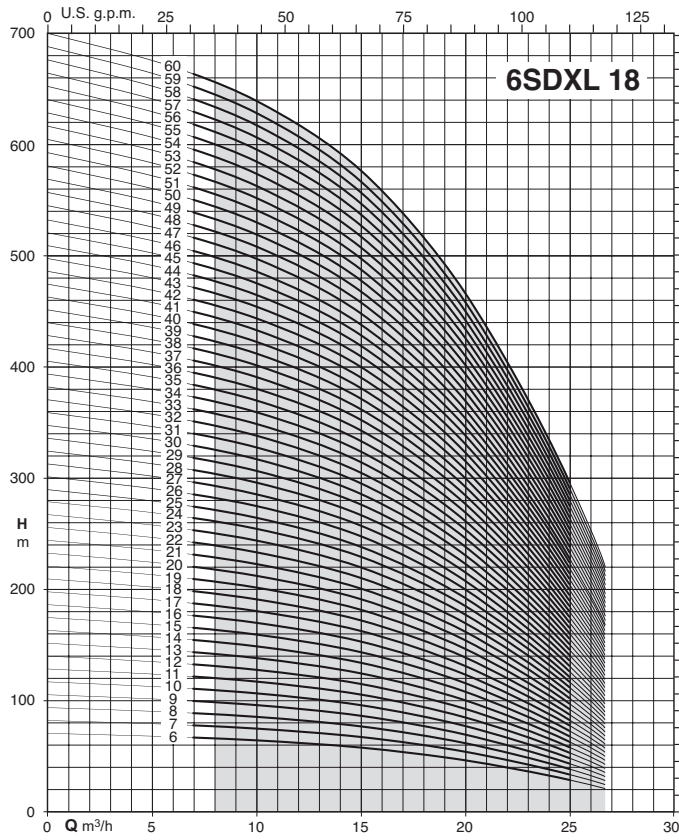
Coverage chart n ≈ 2900 rpm
