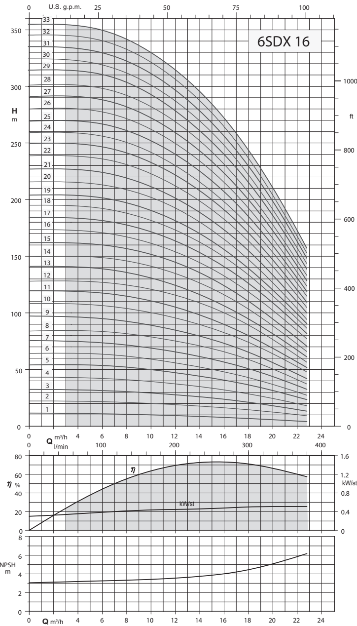
Coverage chart n ≈ 2900 rpm
