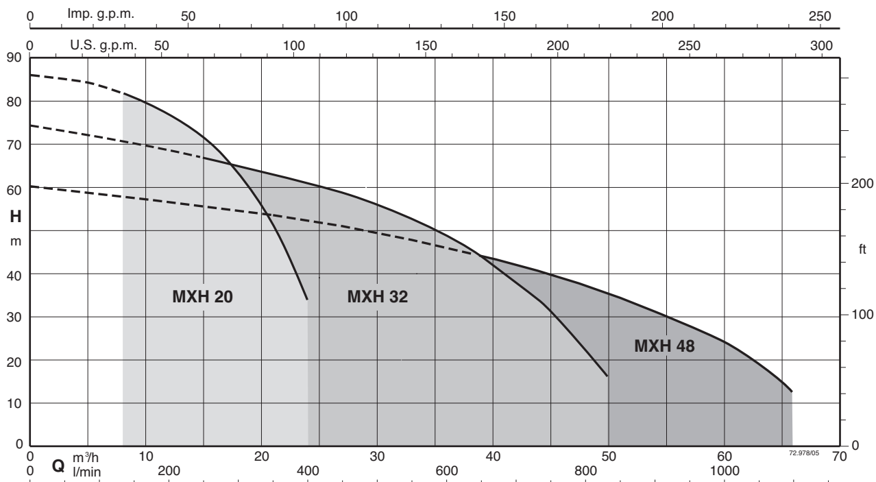
Coverage chart n \approx 2900 rpm
