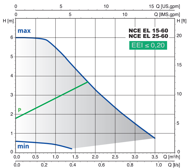
Coverage chart n \approx 2900 rpm
