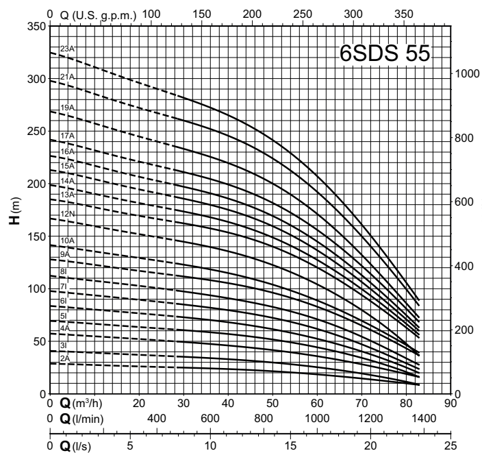
Coverage chart n \approx 2900 rpm
