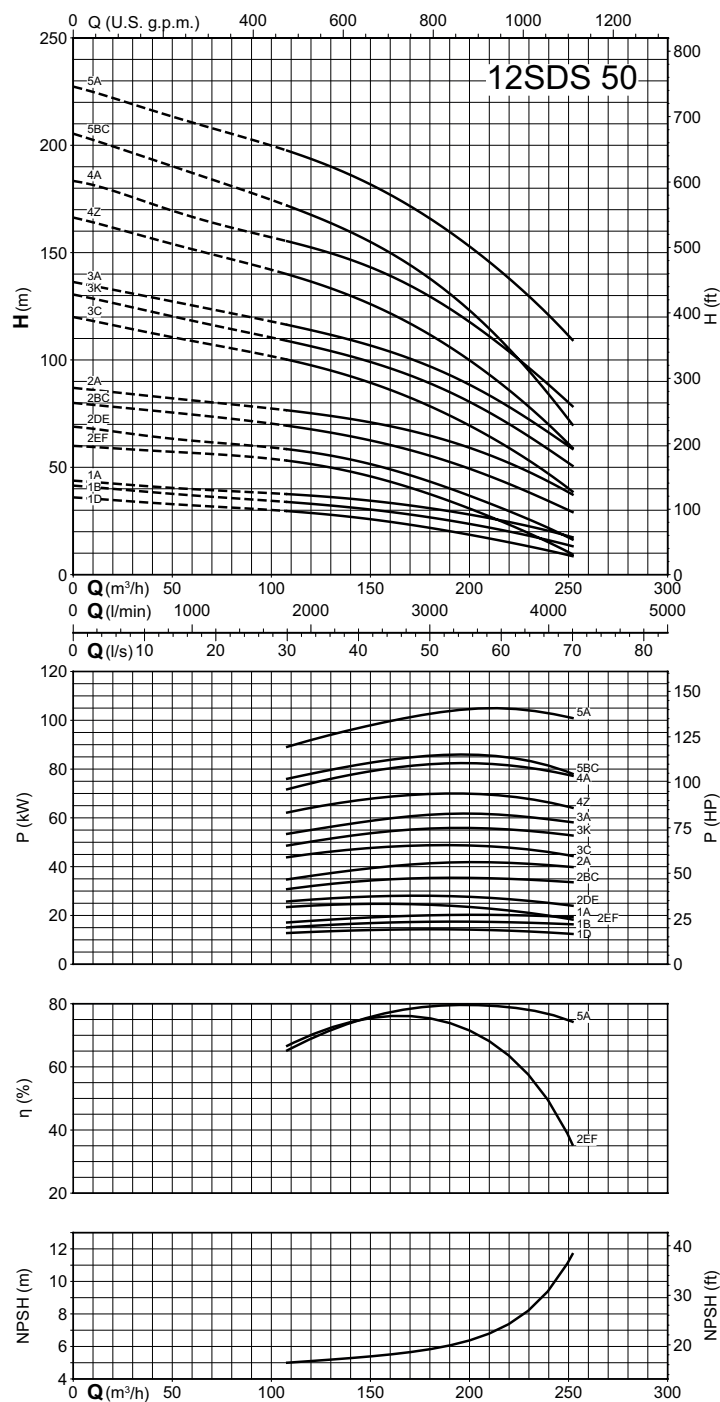
Coverage chart n \approx 2900 rpm
