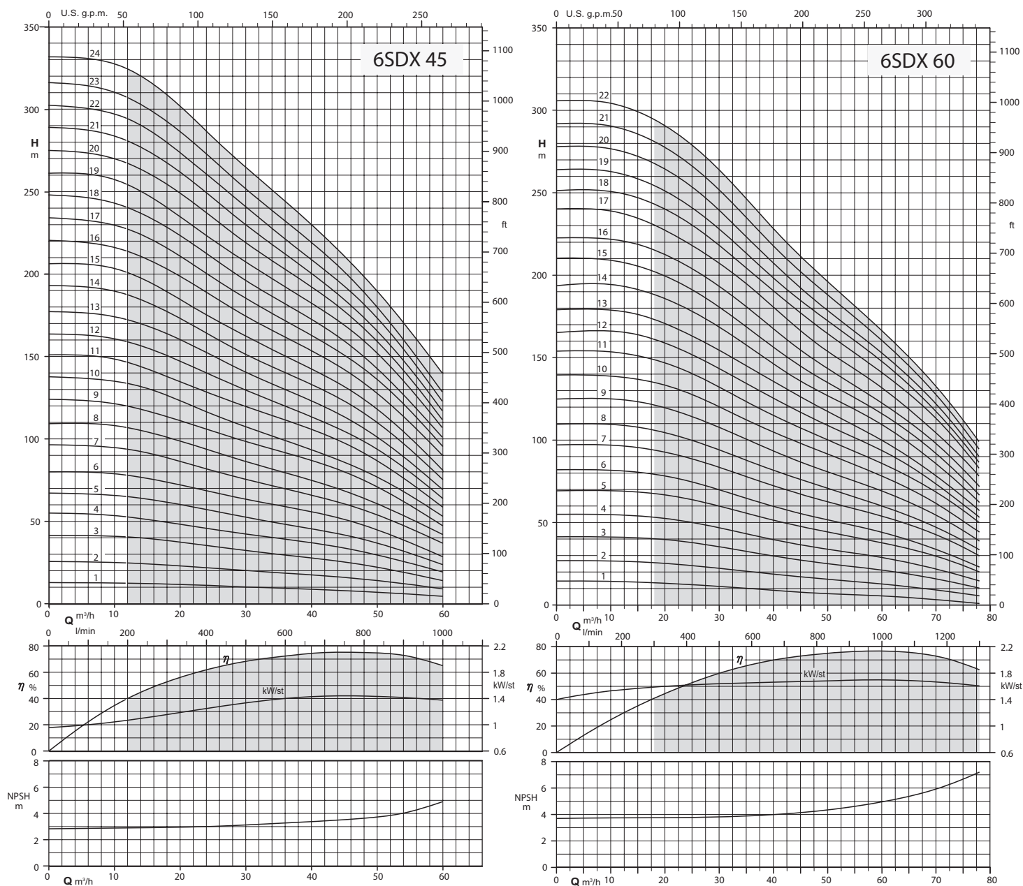
Coverage chart n \approx 2900 rpm
