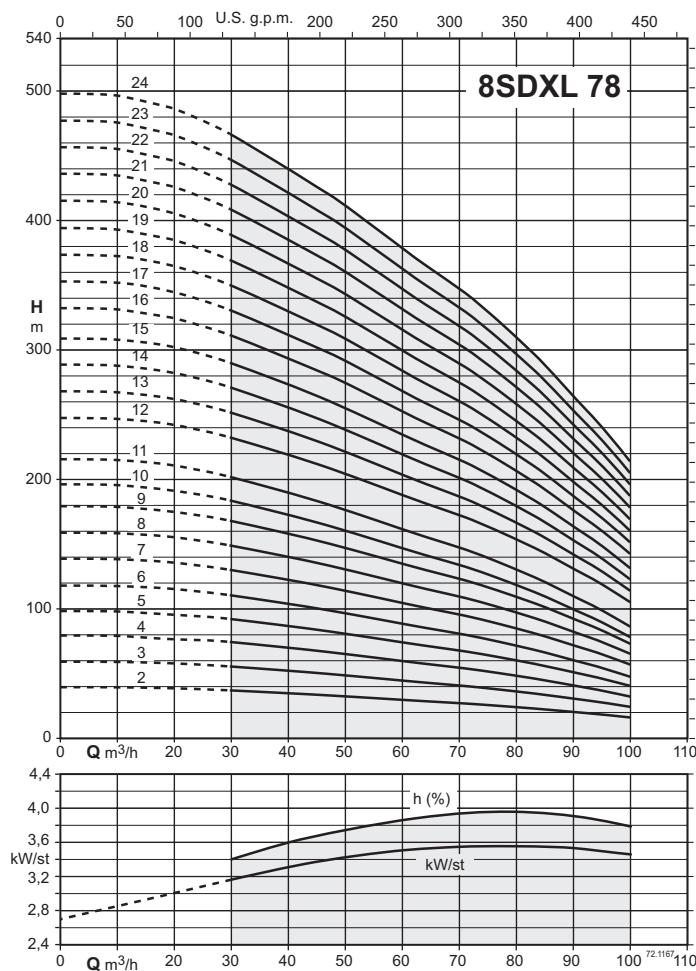
Coverage chart n \approx 2900 rpm
