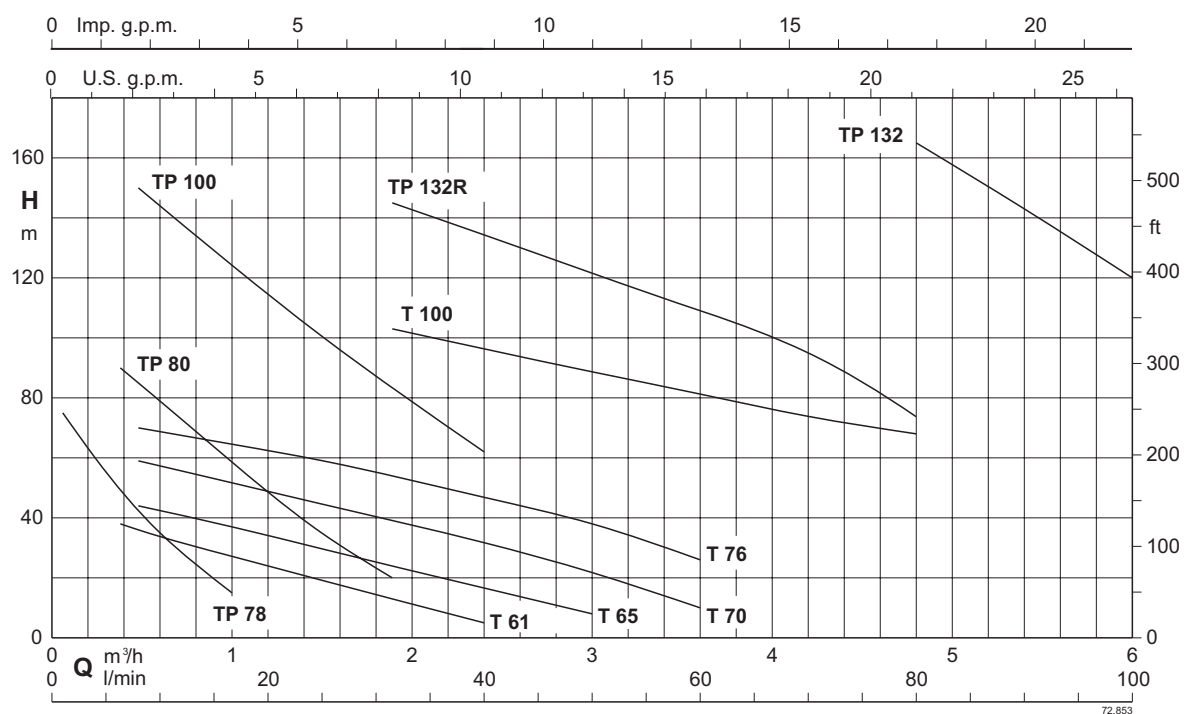
Coverage chart n \approx 2900 rpm
