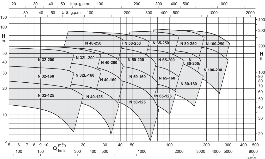
Performances n ≈ 2900 1/min
