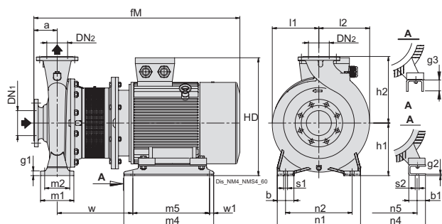
Flanges EN1092-4
