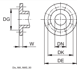
Flanges EN1092-4
