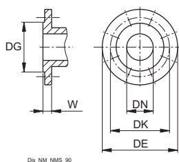
Flanges EN1092-4
