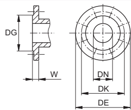
Flanges EN1092-4
