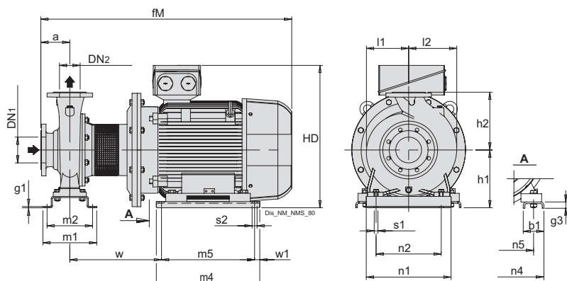
Flanges EN1092-4
