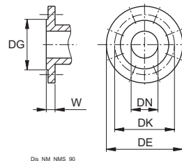
Flanges EN1092-4
