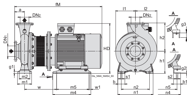
Flanges EN1092-4
