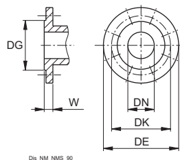
Flanges EN1092-4
