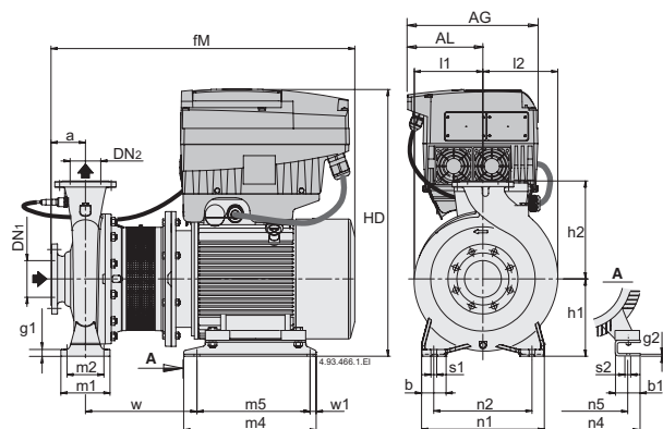
Flanges EN1092-4
