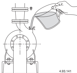
Fig. 3 Filling.
